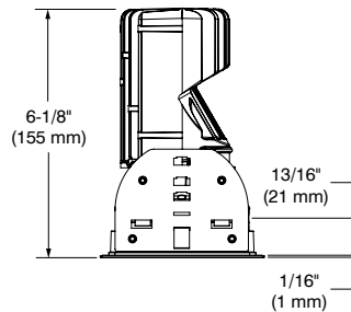
WITH FLANGE
