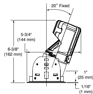
WITH FLANGE
